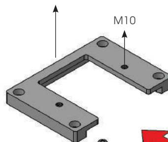
REMOVABLE PLATE 150
